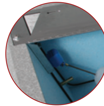
Folding hood for easy float adjustment with stainless steel hinge
